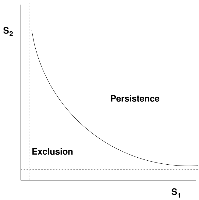
Figure 10: Alternating hosts
