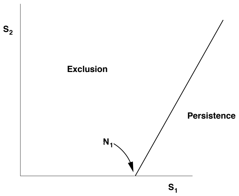
Figure 11: Inhibitory hosts
